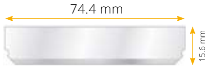
74.4 x 15.6 x 0.84 mm
