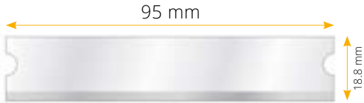
95 x 18.8 x 0.91 mm
